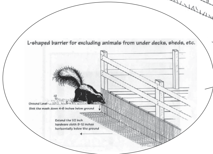
Deck/Shed "L-Shaped Barrier"
